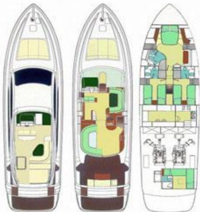
Fly Bridge
