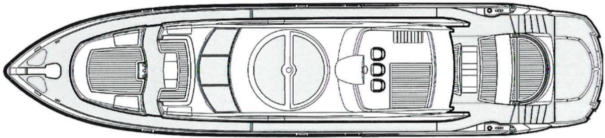
Sports flybridge deck
